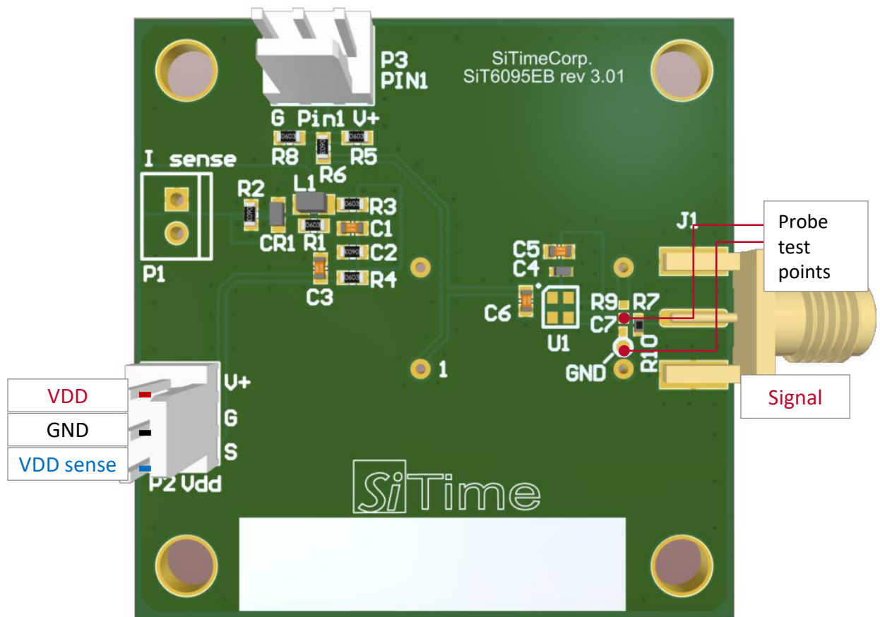
Figure A2: SiT6095EB layout
