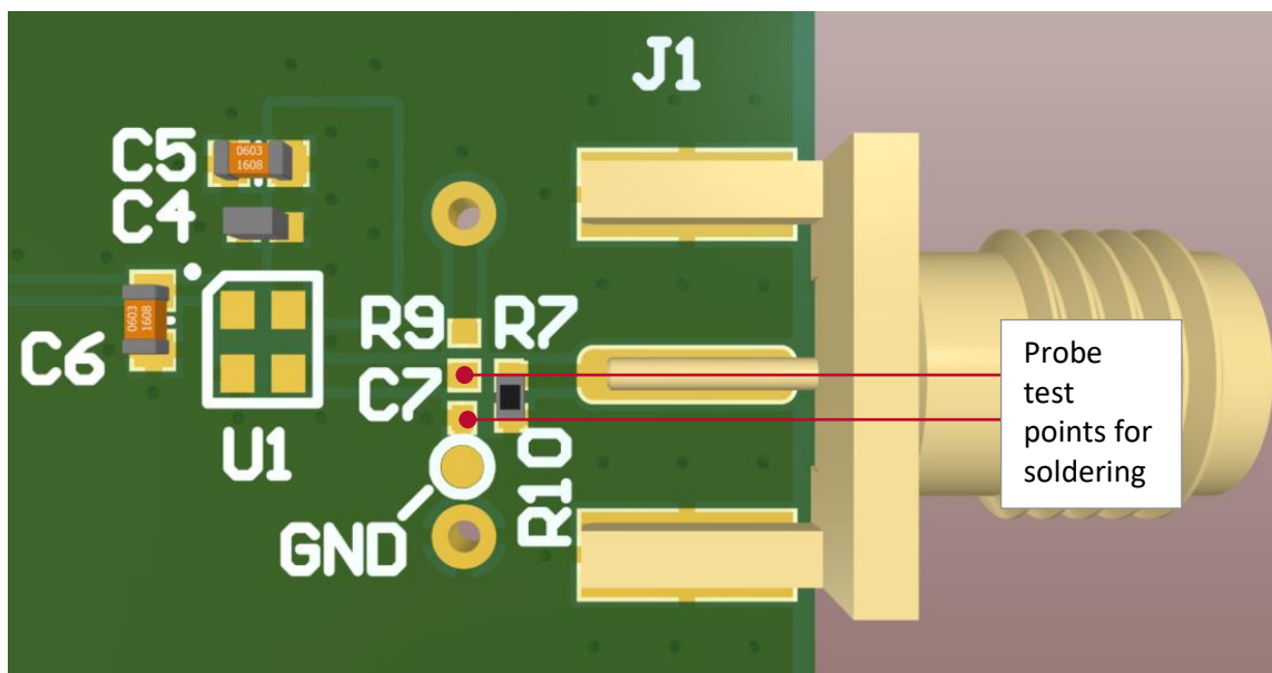
Figure 1: Recommended points for soldering probe head
