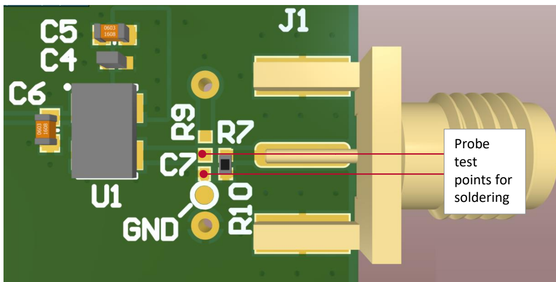
Figure 1: Recommended points for soldering probe head
