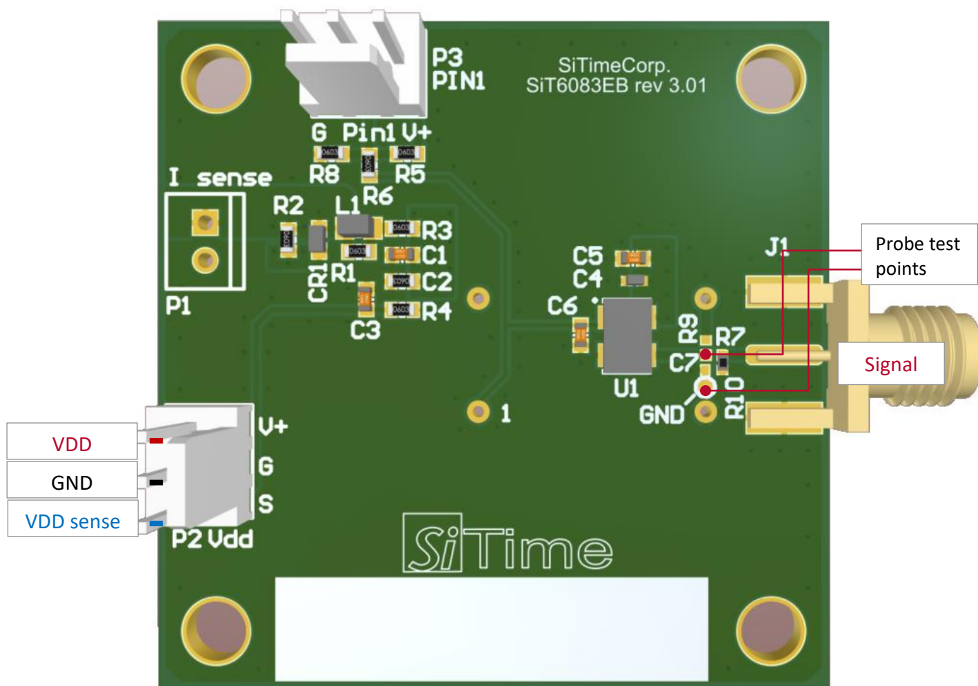
Figure A2: SiT6083EB layout
