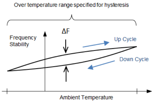
Figure 19. Illustration of hysteresis, where ΔF is max frequency difference between up and down cycles across temperature
