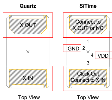
Figure 3. CS00117 Footprint Compatibility with Quartz XTAL Footprint 6
