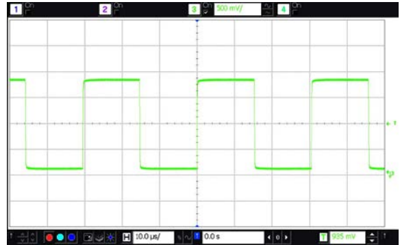
Figure 14. LVC MOS Output Waveform ( V_{swing} = 1.8\text{V} , CS00117AI-H4-DCC-32.770)
