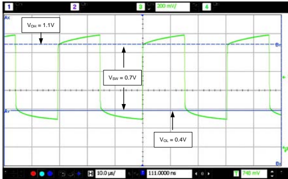
Figure 13. NanoDrive™ Output Waveform ( V_{OH} = 1.1\text{V} , V_{OL} = 0.4\text{V} ; CS00117AI-H4-D14-32.770)
