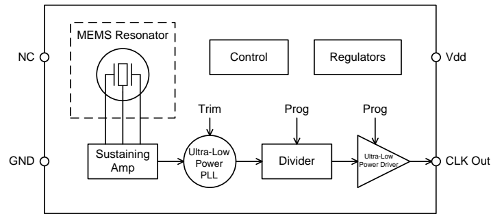
Figure 2. CS00117 Block Diagram
