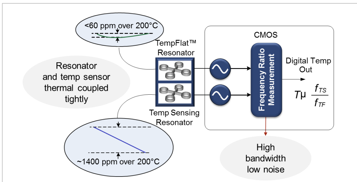
Figure 2: DualMEMS resonators temperature sensing with <30 \mu\text{K} resolution and noiseless temperature compensation
