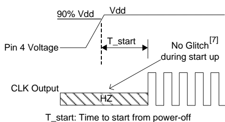
Figure 4. Startup Timing (OE/ \overline{\text{ST}} Mode)
