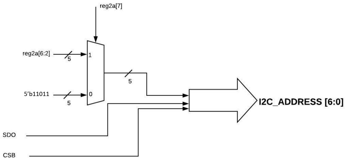
Figure 36. I 2 C Addressing Scheme for Cascade
