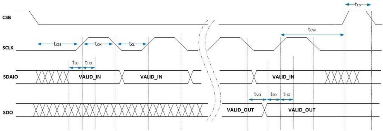
SPI Slave revC Timing Diagram
