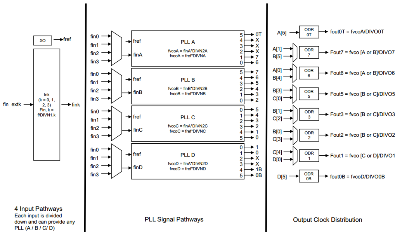
Figure 11. Overall Hierarchy of Clocks
