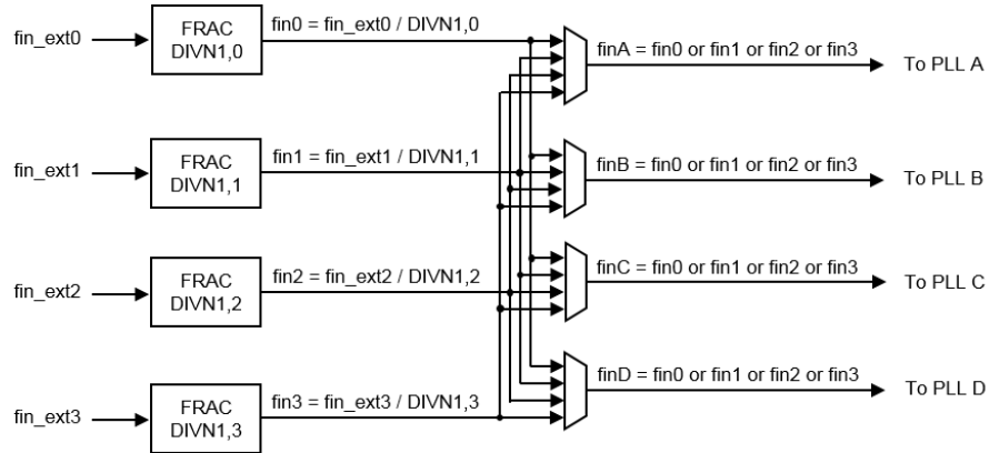
Figure 12. Input Clock Distribution
