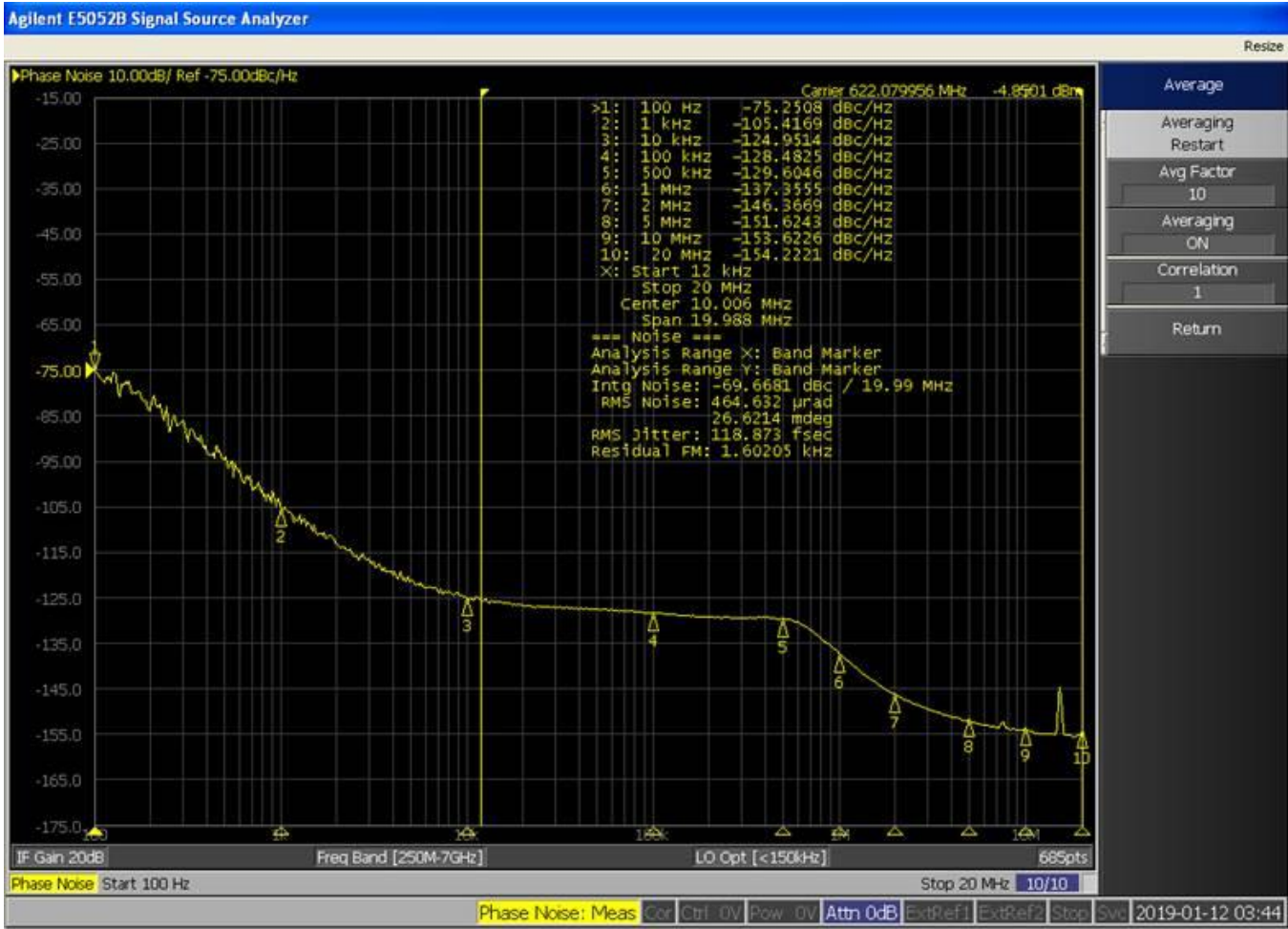
Figure 3. Representative Phase Noise Measurement: F_{OUT} = 622.08\text{ MHz} , F_{IN} = 10\text{ MHz} , BW = 100 Hz
