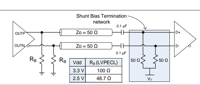
Figure 23. Recommended LVPECL and FlexSwing [18] Termination when AC-coupled
