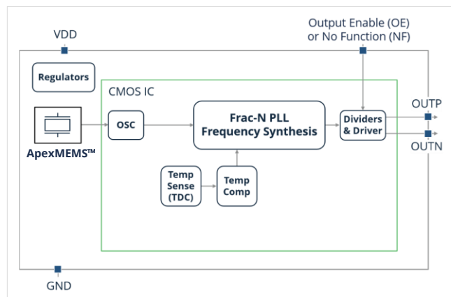
Figure 1. SiT9377 Block Diagram
