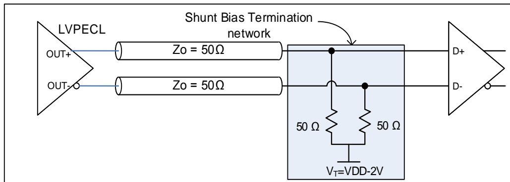
Figure 13. LVPECL with DC-coupled Parallel Shunt Load Termination
