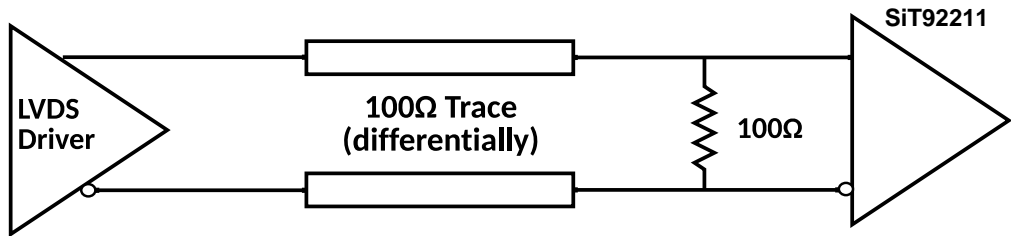
Figure 14. Termination scheme for DC coupled LVDS
