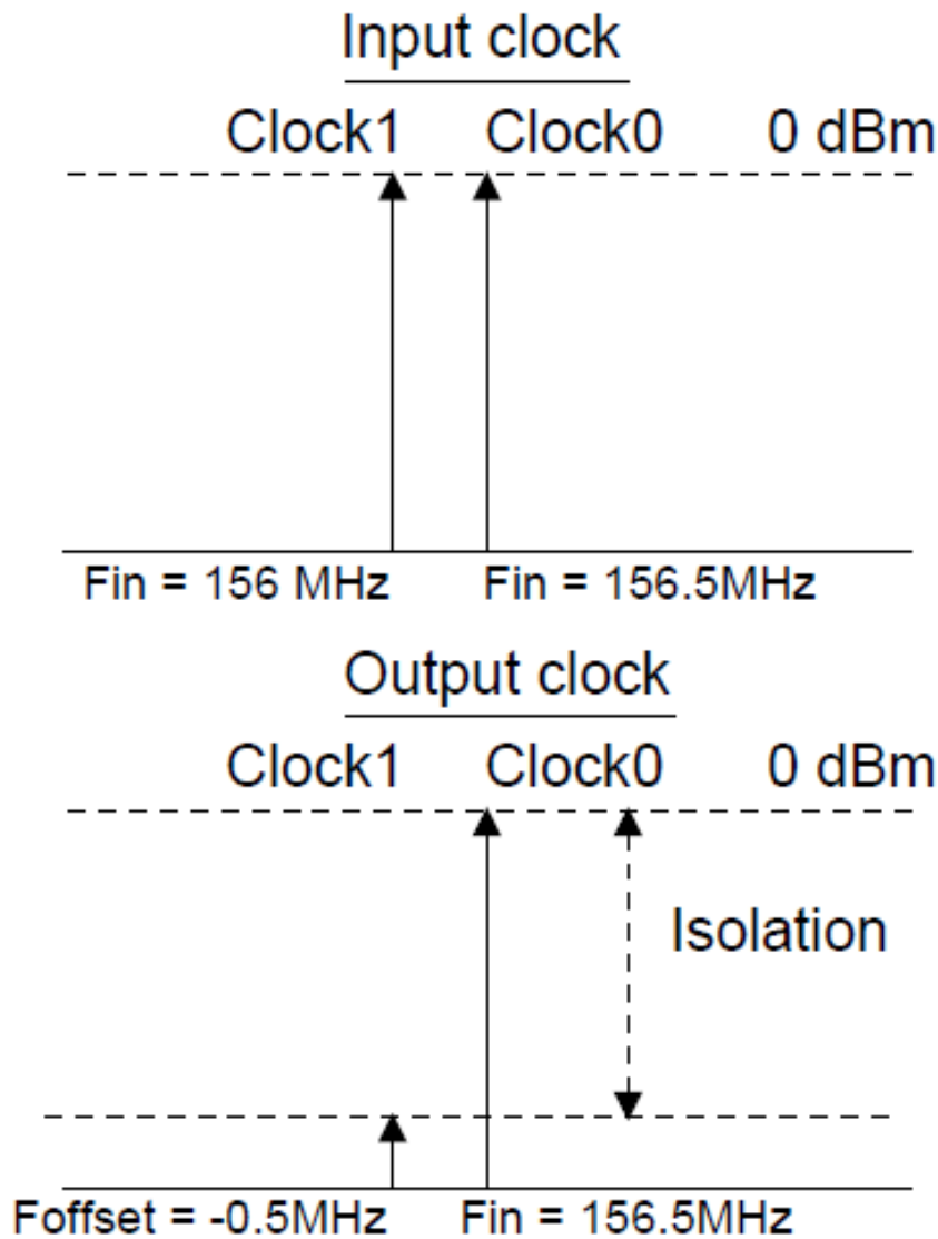
Figure 47 Parameter definition of isolation
