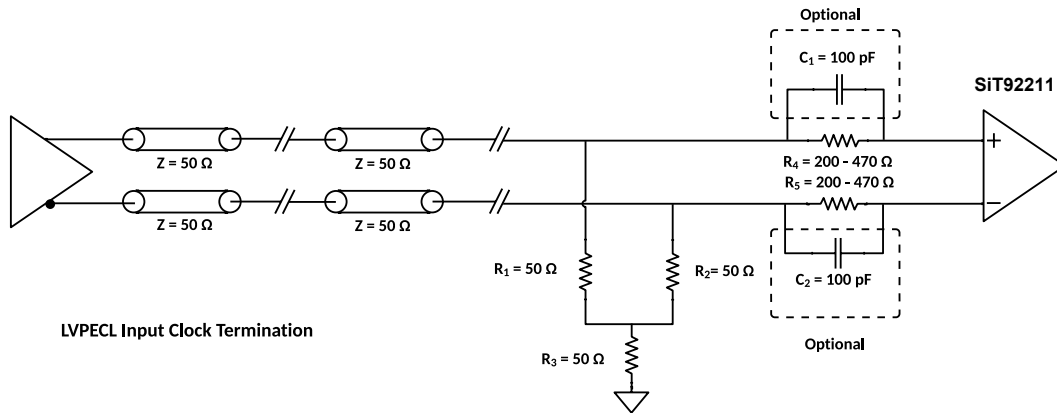
Figure 38 LVPECL termination with hot swap protection
