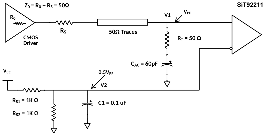
Figure 9 DC coupled LVCMOS input clock with series RC termination – configuration 3
