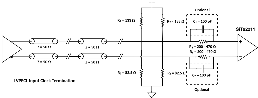
Figure 37. LVEPCL termination with hot swap protection
