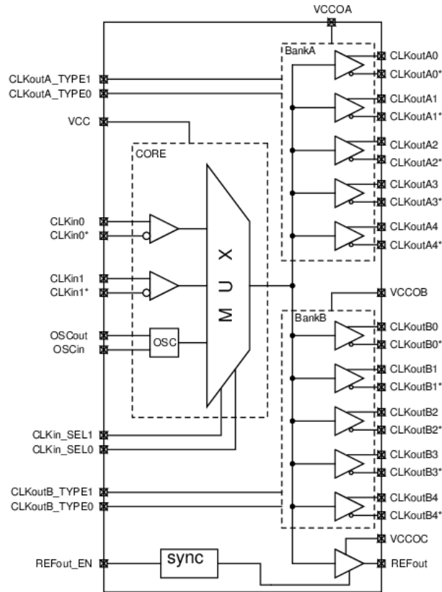
Figure 1. SiT92211 Block Diagram
