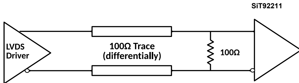
Figure 14 Termination scheme for DC coupled LVDS
