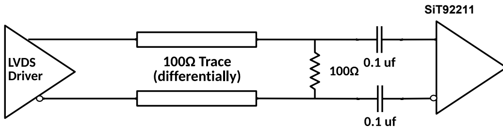
Figure 19 Termination scheme for AC coupled LVDS
