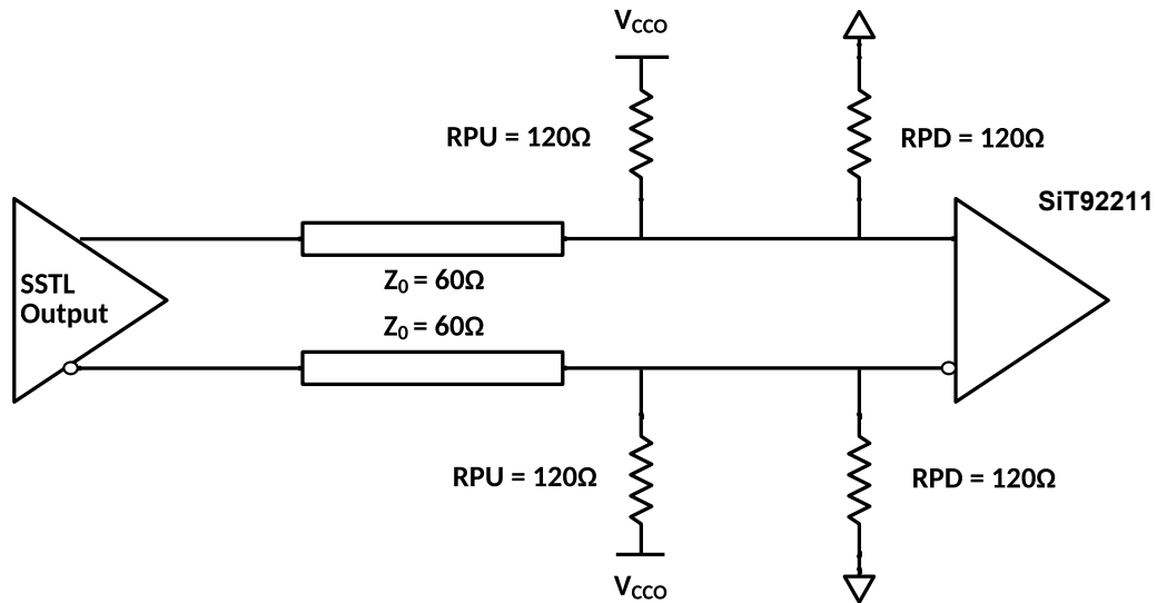
Figure 18 Example of input clock termination for SSSL clock.
