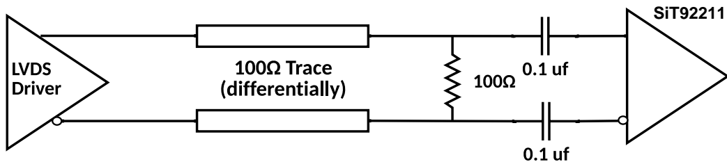
Figure 19. Termination scheme for AC coupled LVDS
