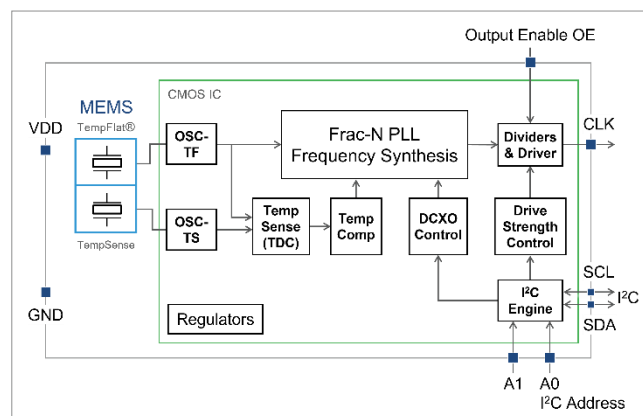
Figure 1. SiT5543 Block Diagram
