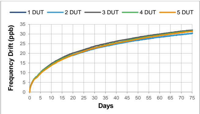
Figure 19. Frequency Drift
