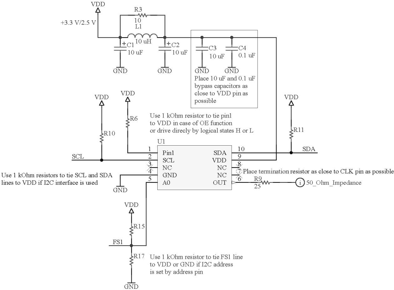
Figure 46. DCTCXO schematic example
