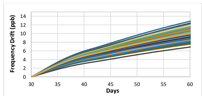
Figure 21. Frequency drift after 30 days [15]
