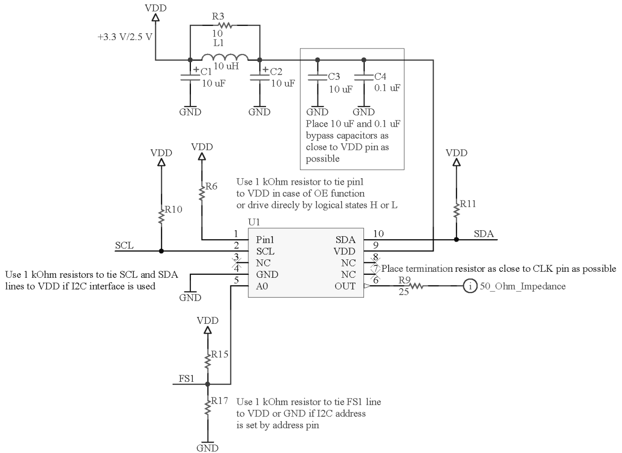
Figure 60. DCTCXO schematic example
