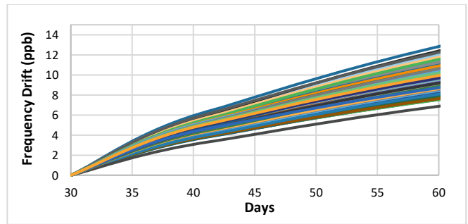
Figure 27. Frequency drift after 30 days [15]
