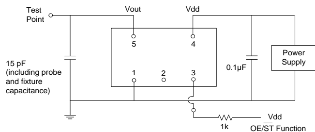
Figure 2. Test Circuit [6]
