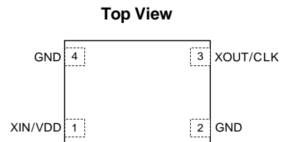
Figure 1. Pin Assignments
