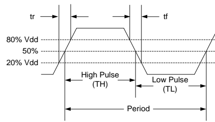
Figure 3. Waveform [10]
