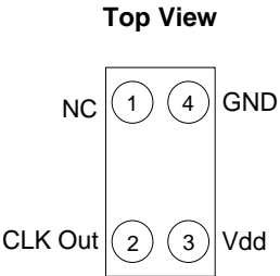
Figure 1. Pin Assignment
