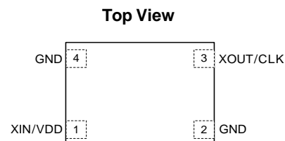
Figure 1. Pin Assignments
